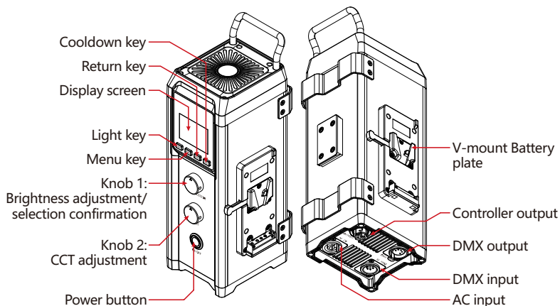
Control Box
