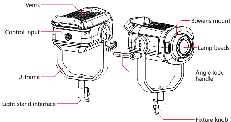
Lamp Head
