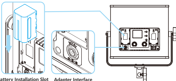
Battery Installation Slot
